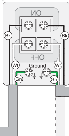
MOTOR (Wired 220V)
